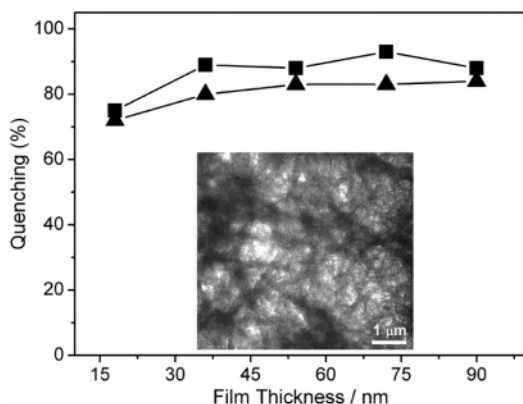
Figure 2. Thickness dependence of fluorescence quenching efficiency of ACTC films. The quenching was tested upon exposing the film to saturated vapor of TNT ( \blacktriangle ) and DNT ( \blacksquare ) for 60 s. The inset is a TEM image of a thin film of ACTC cast on silicon oxide from 2 mM THF solution.
